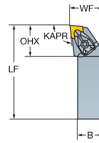
DCLNR/L 95.0°
