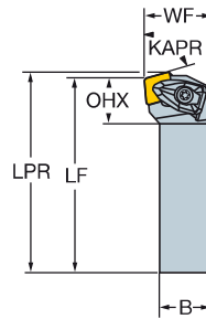
DCKNR/L 75.0°
