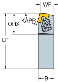
DCBNR/L 75.0°
